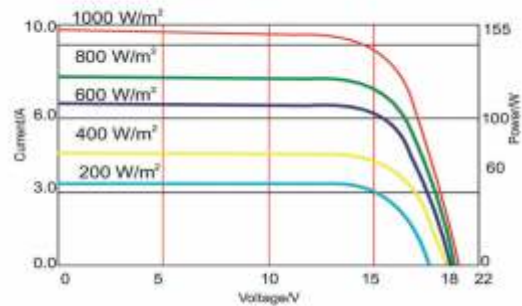
I-V CURVE
