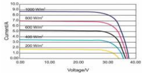
I-V CURVE
