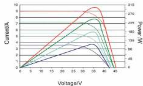
I-V CURVE
