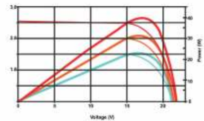
I-V CURVE
