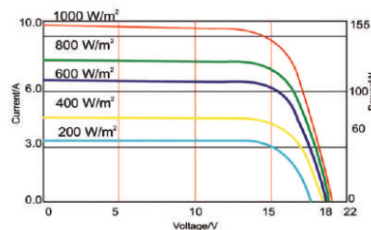
I-V-CURVE
