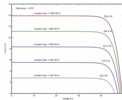
I-V-CURVE
