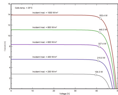
I-V-CURVE
