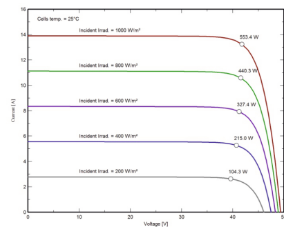
I-V-CURVE
